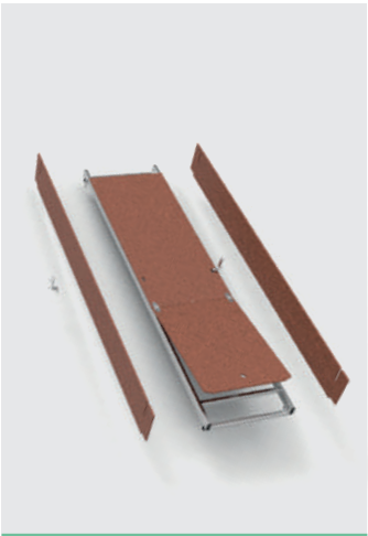
PIANO LAVORO C/ BOTOLA + TAVOLE LUNGHE Platform with trapdoor+ long toeboards
