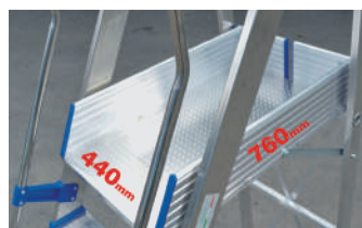
Workplatform 760x440 mm in grooved aluminum sheet, with toaboard
